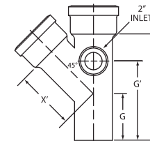
Wye w/Right Hand Side Inlet
