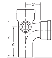
Sanitary Tee w/Left Hand Side Inlets
