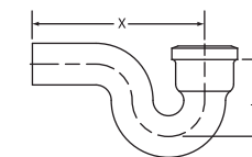
"P" Trap
